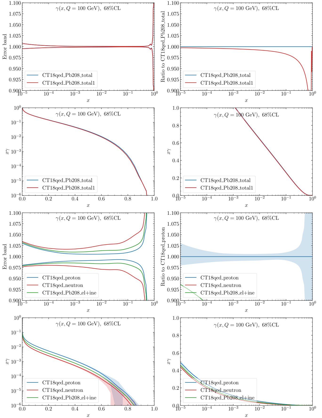
FIG. 1. compare: CT18qed_proton_CT18qed_neutron_CT18qed_Pb208_el+ine_Q100GeV_07_xpho_logx
