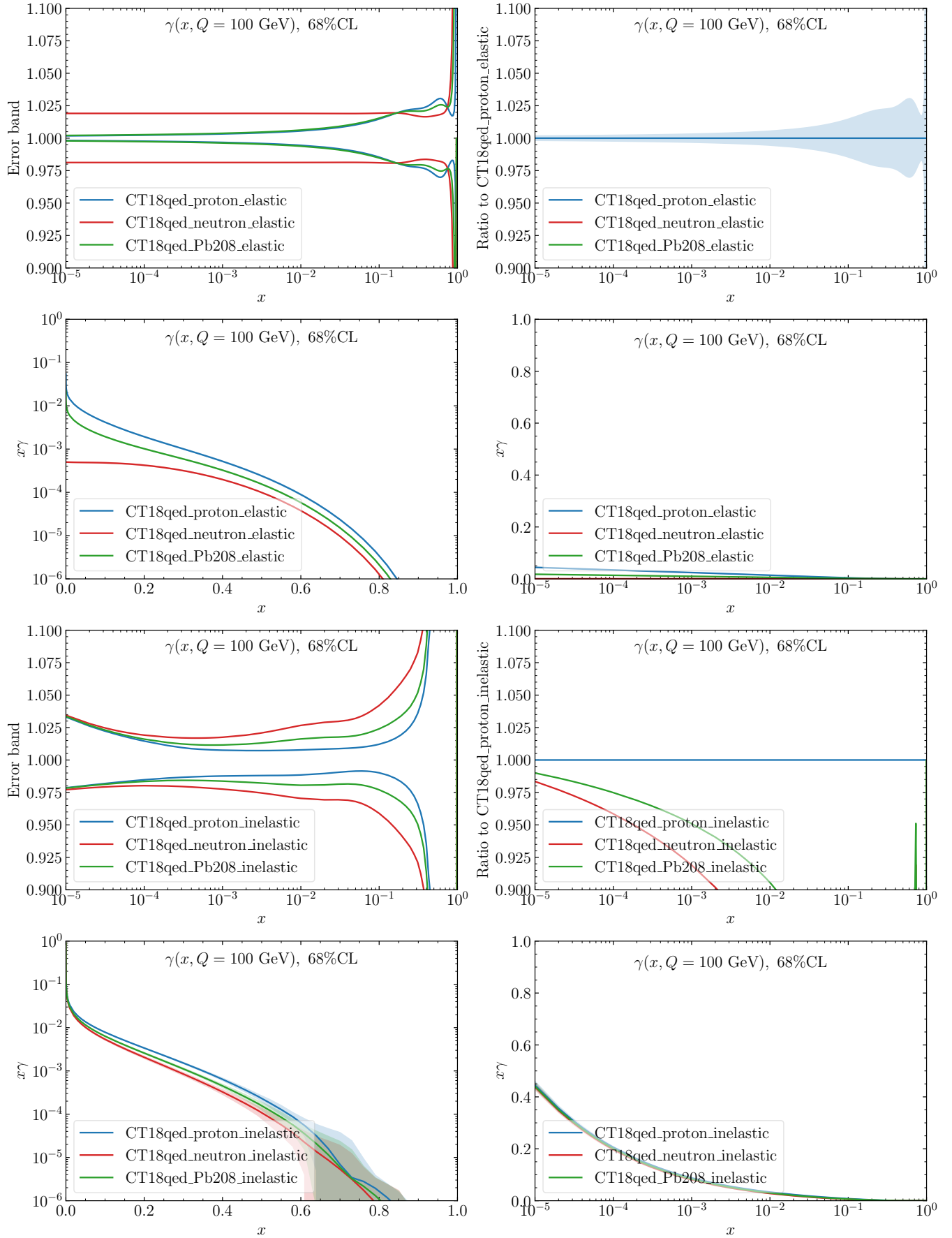
FIG. 2. compare: CT18qed_proton_inelastic_CT18qed_neutron_inelastic_CT18qed_Pb208_inelastic_Q100GeV_07_xpho_logx
