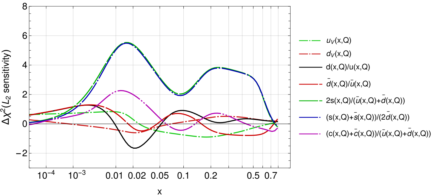
CT18Z NNLO, CcfrNuChXN (126), Q=2 GeV
