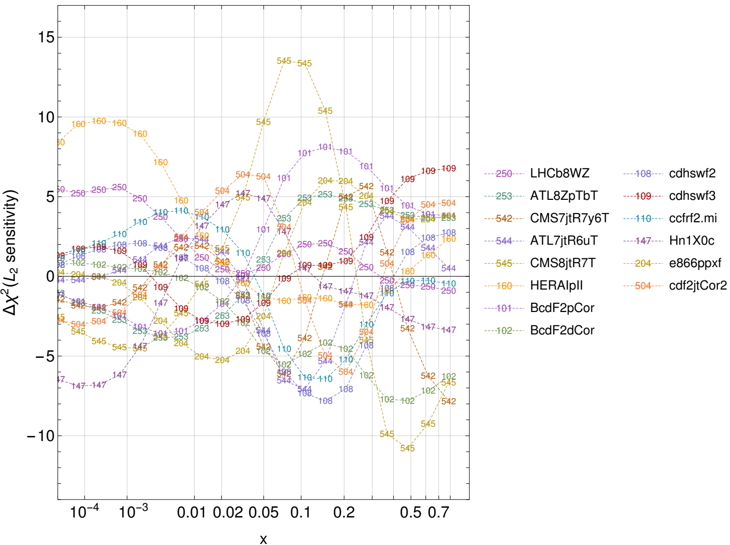
CT18 NNLO, c(x, 100 \text{ GeV})
