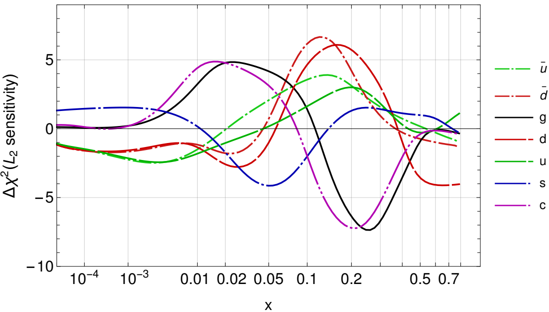
CT18 NNLO, ccfrf2.mi (110), Q=2 GeV
